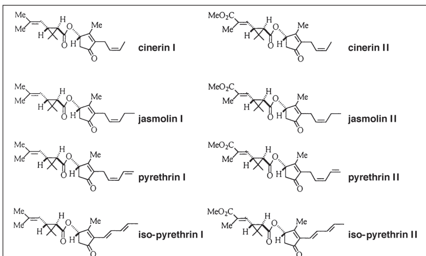
Figure 1. Biologically active rethrin constituents of pyrethrum and thermally induced isomers of pyrethrins.
